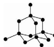
graphene
